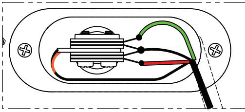
TOGGLE SWITCH
